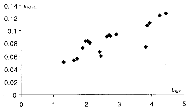
Fig. 7. Actual error versus the h/r criterion for elements of 'reasonable' shape (aspect ratio k from 0.25 to 4). Results for 18 meshes.
