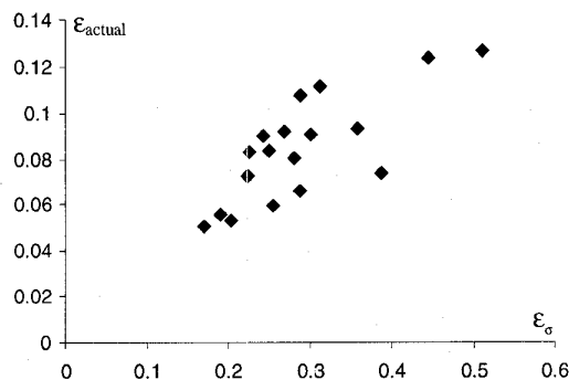
Fig. 6. Actual error versus the singular value estimate for elements of 'reasonable' shape (aspect ratio k from 0.25 to 4). Results for 18 meshes.
